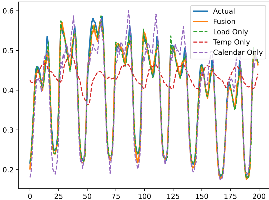
Fusion vs Unimodal Models
